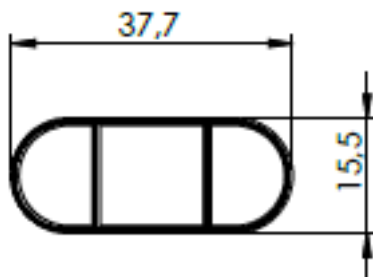
OBLONGO 37,7x15,5 x1,0MM
