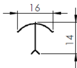
CANTONEIRA REDONDA
