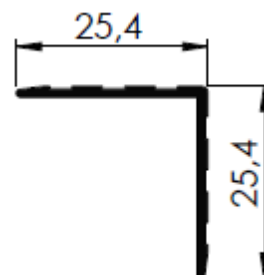
CASE 04 25,4 X25,4MM
