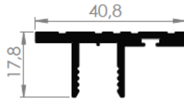
TRANSPASSE 40,8X17,8MM
