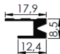
CASE 06 17,9 X12,4MM
