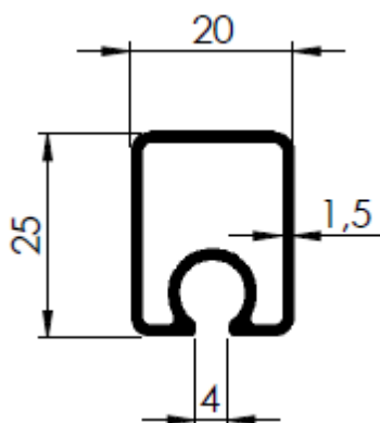
TRAVA TELA 25 X 20 X 1,5MM
