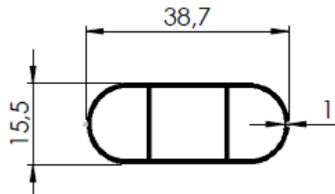
OBLONGO 38,7x15,5x1,0MM
