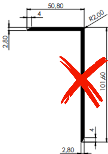
CANTONEIRA L BAU 4X2X2,8MM
