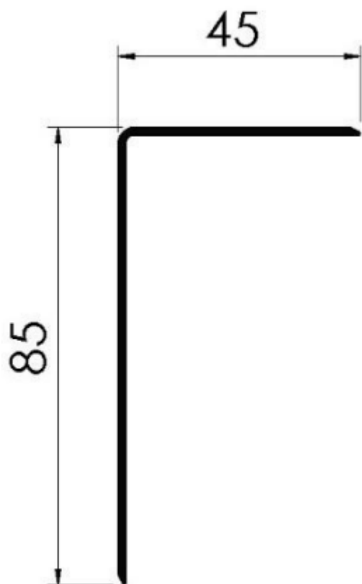
CANTONEIRA 85X45X1,4MM
